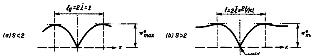
Fig. 5. Form of shell distortion caused by residual stresses from circumferential welding.
