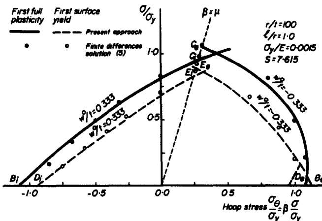
Fig. 7(b). Elastoplastic interactions between axial and hoop stresses for a shell with S = 7.615 .
