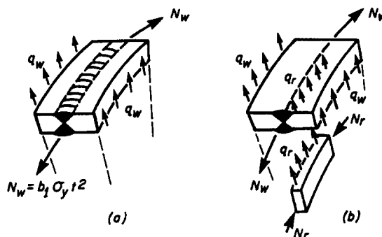
Fig. 4. Nature of weld shear q_w induced by residual stresses arising from circumferential welding.
